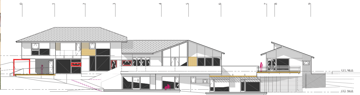
main house FRONT ELEVATION - sea facing side
